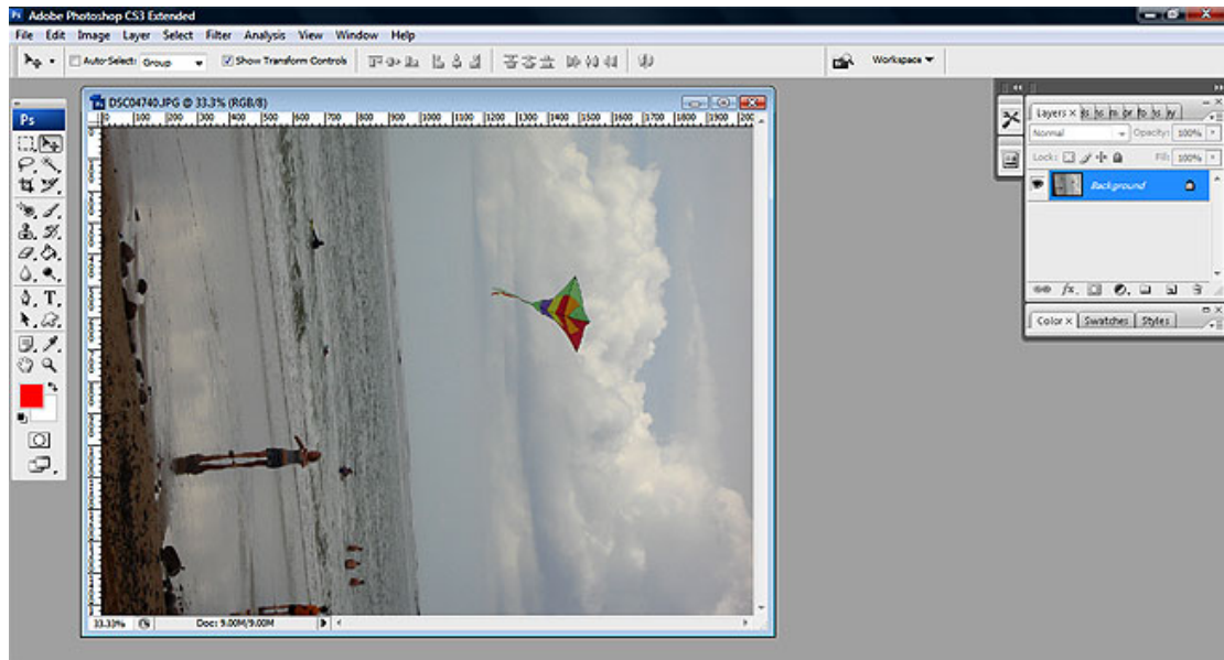
Figure 1.2 Photoshop Interface.
