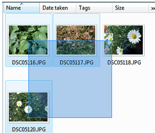
Figure 10.2 Selection box
