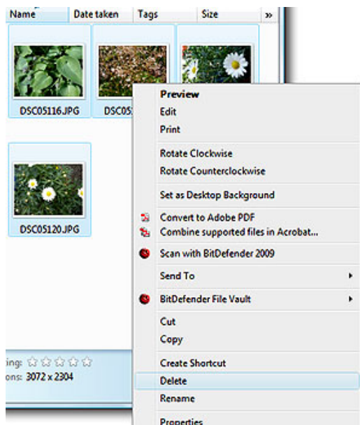
Figure 10.3 Delete option.
